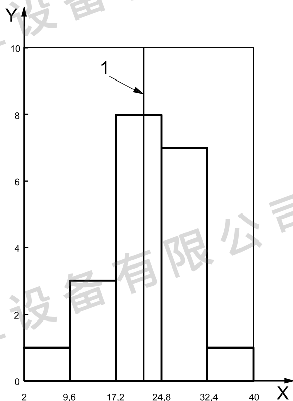
d) Sample B, type 1A test piece
