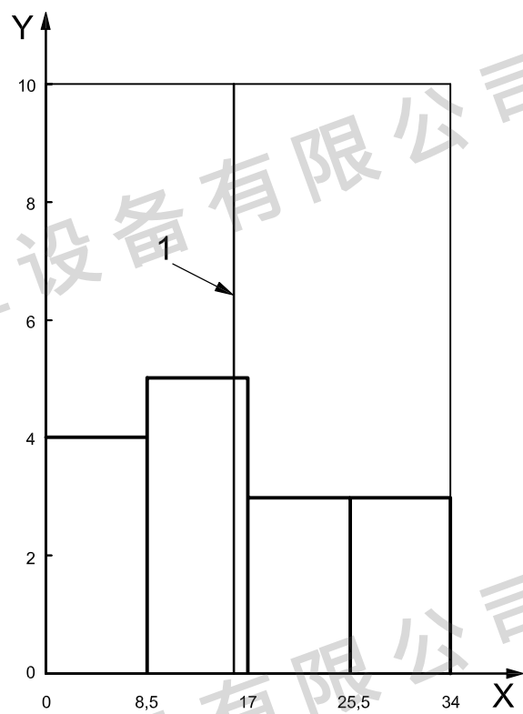
b) Sample A, type 1A test piece
