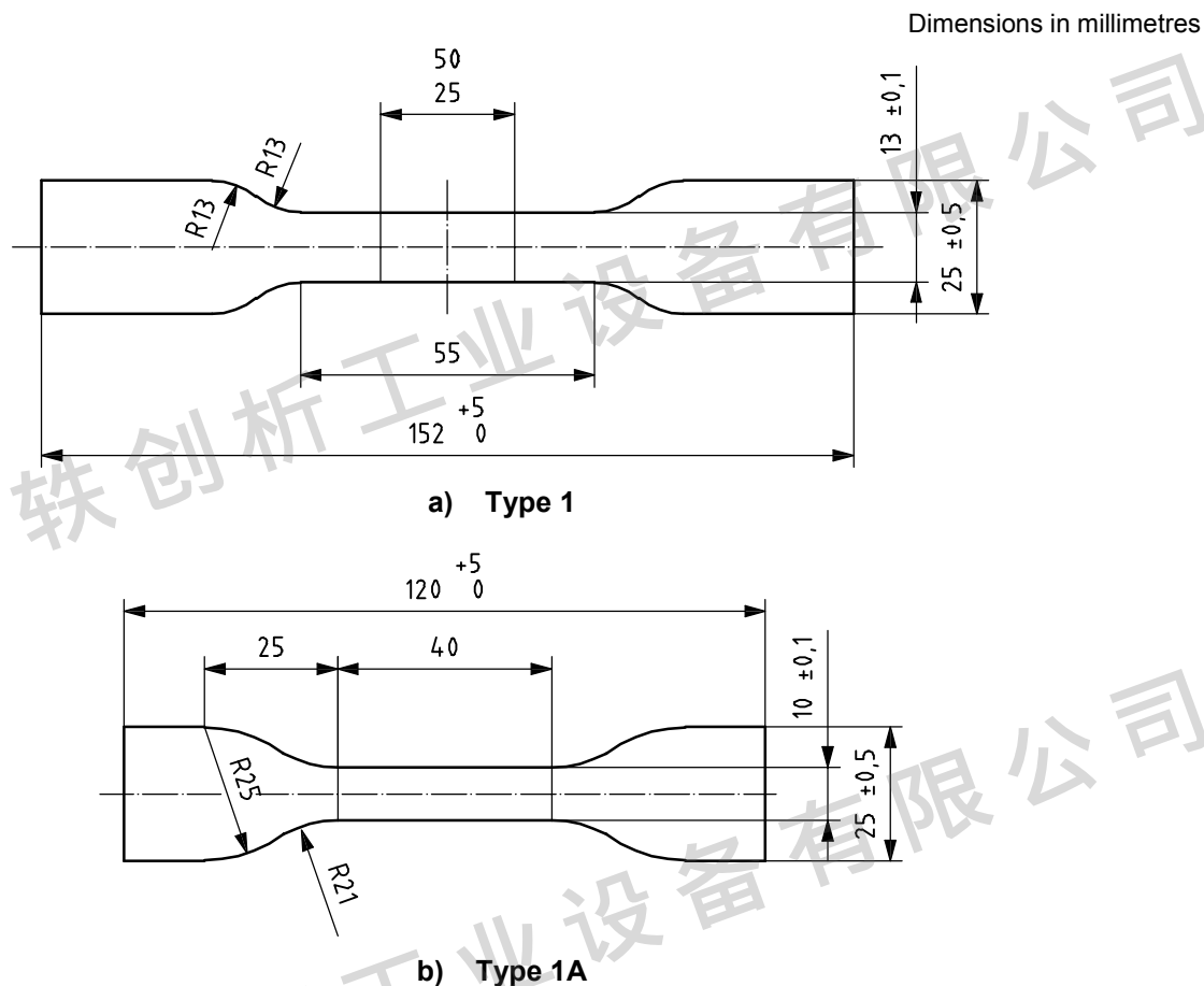
Figure 1 — Test-piece cutters
