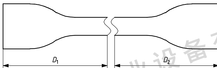
Figure A.2 — Measurement of position of breaking point
