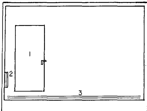
FIG. A1 Typical Salt Spray Cabinet.
