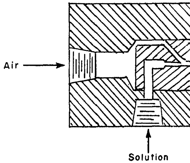
FIG. A3 Typical Spray Nozzle.
