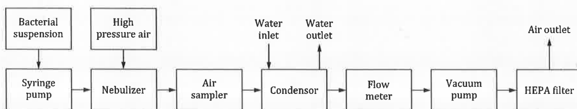
Figure B.1 — Principle of BFE test apparatus
